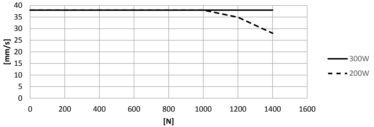
2 x DL45 (equally loaded) with CBD6S
